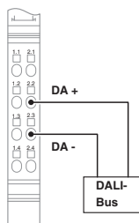
Connection diagram
