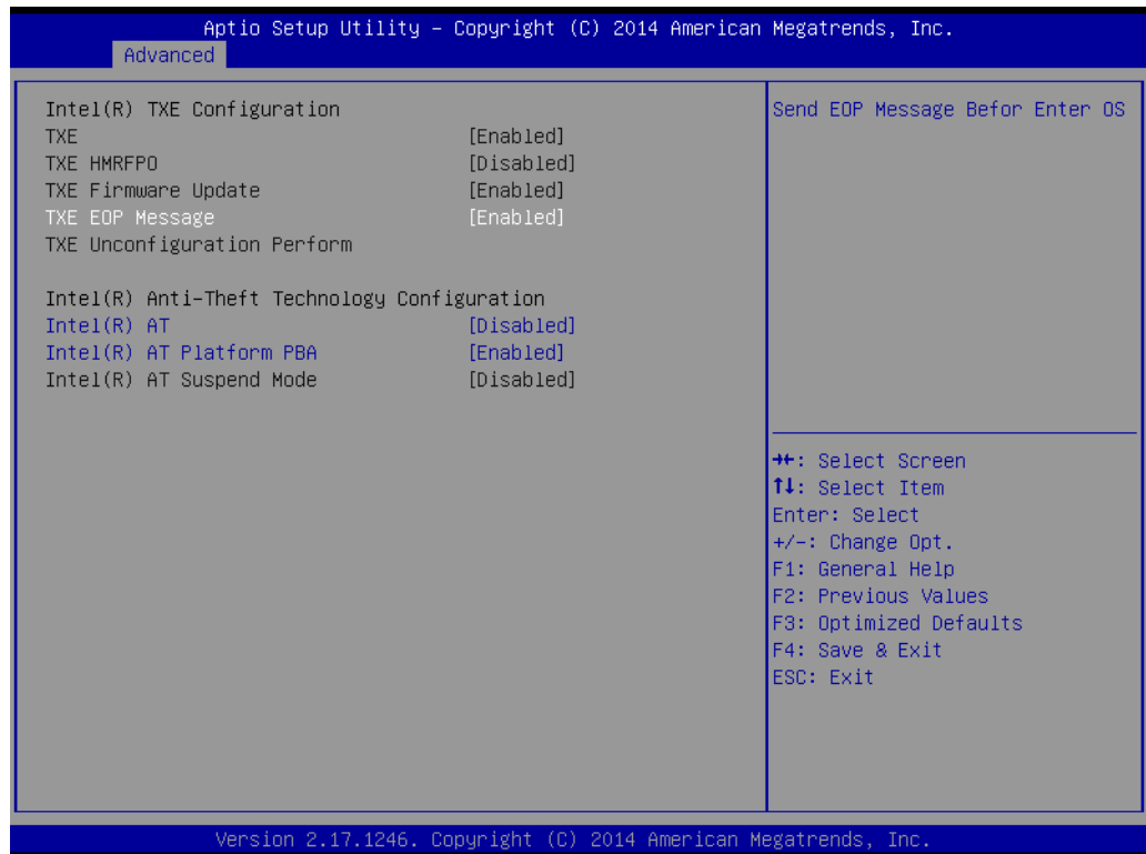
Figure 3.24 Security Configuration
